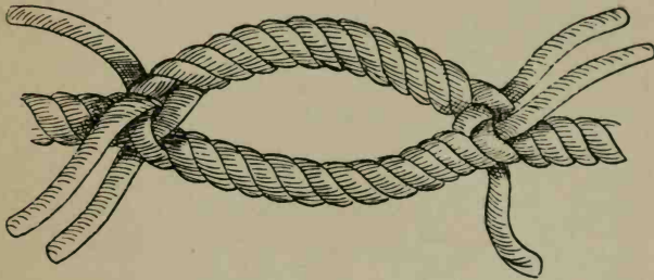
FIG. 109.—Cut splice.
